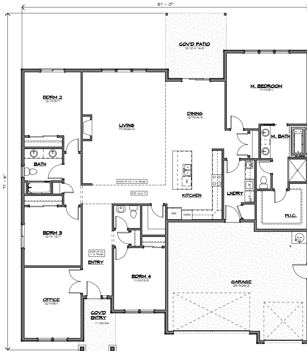
Main Floor Plan - 2697 SF 1/4" = 1'-0"
